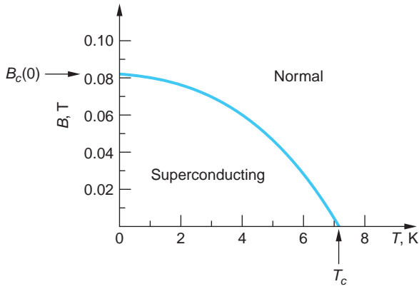
FIGURE 10-47 Variation of the critical temperature with magnetic field for lead. Note that B_c approaches zero as T approaches T_c .
